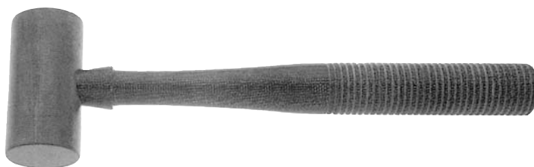
100-604-12 18,0 cm length, 30 mm, 125 g (4 oz) Material Ferozell can be sterilized in an autoclave at 3 bar overpressure (143°C)
