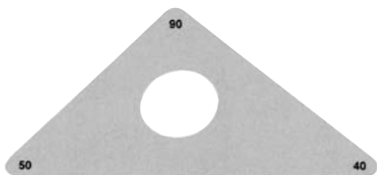
119-516-04 Triangular Positioning Plate 90^{\circ}/50^{\circ}/40^{\circ}
