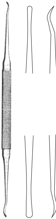
160-227-19 Kleinert Kutz Elevator and Dissector 195 mm 2 mm x 3 mm Sharp ends
