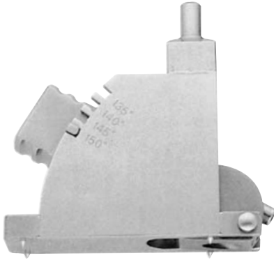
118-533-04 Drill Guide adjustable to 135° / 140° / 145° / 150°
