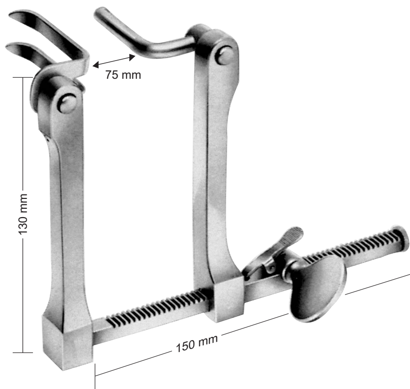
160-185-15 Caspar Retractor Frame 160-186-15 Caspar Retractor Frame (hinged)
