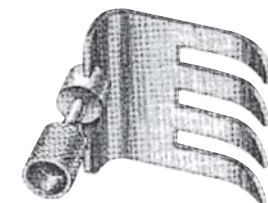
160-180-01 Taylor Laminectomy Blades 160-180-02 51 mm width x 48 mm depth 160-180-03 64 mm width x 64 mm depth 57 mm width x 76 mm depth
